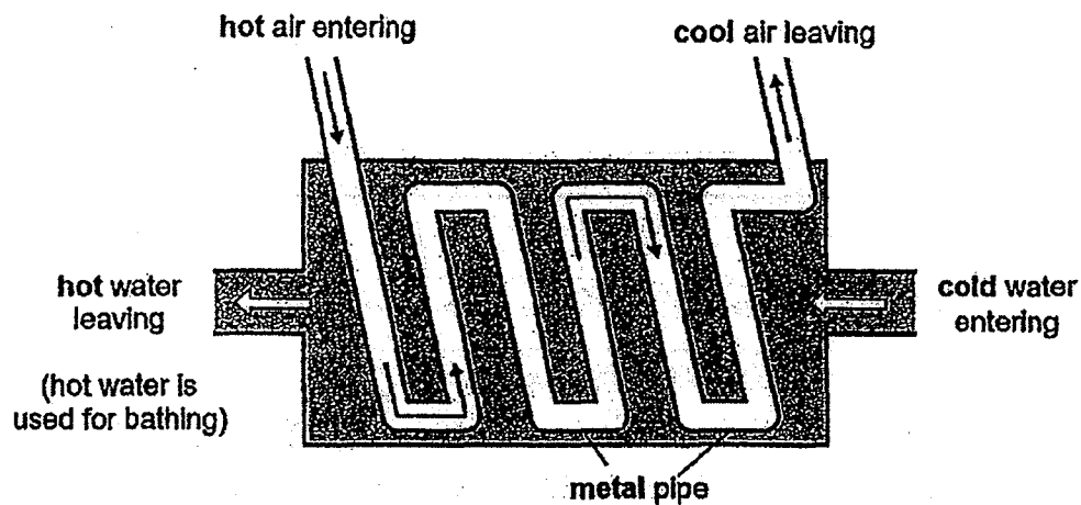
Water Heater
