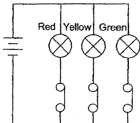
circuit A
