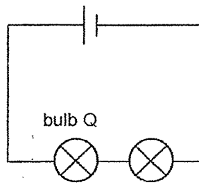
Circuit X
