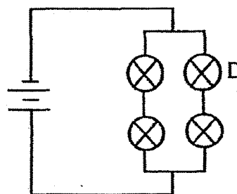
Circuit S
